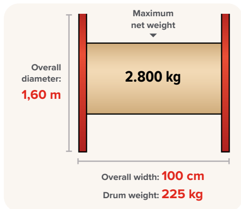
DRUM Ø 1600
