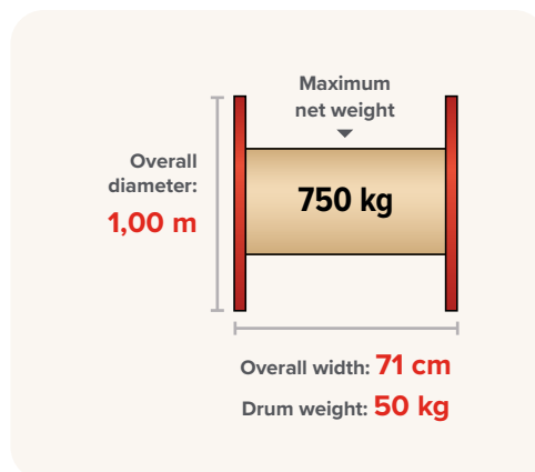
DRUM Ø 1000
