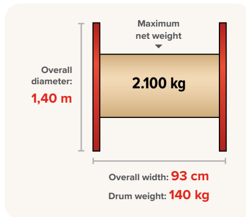
DRUM Ø 1400
